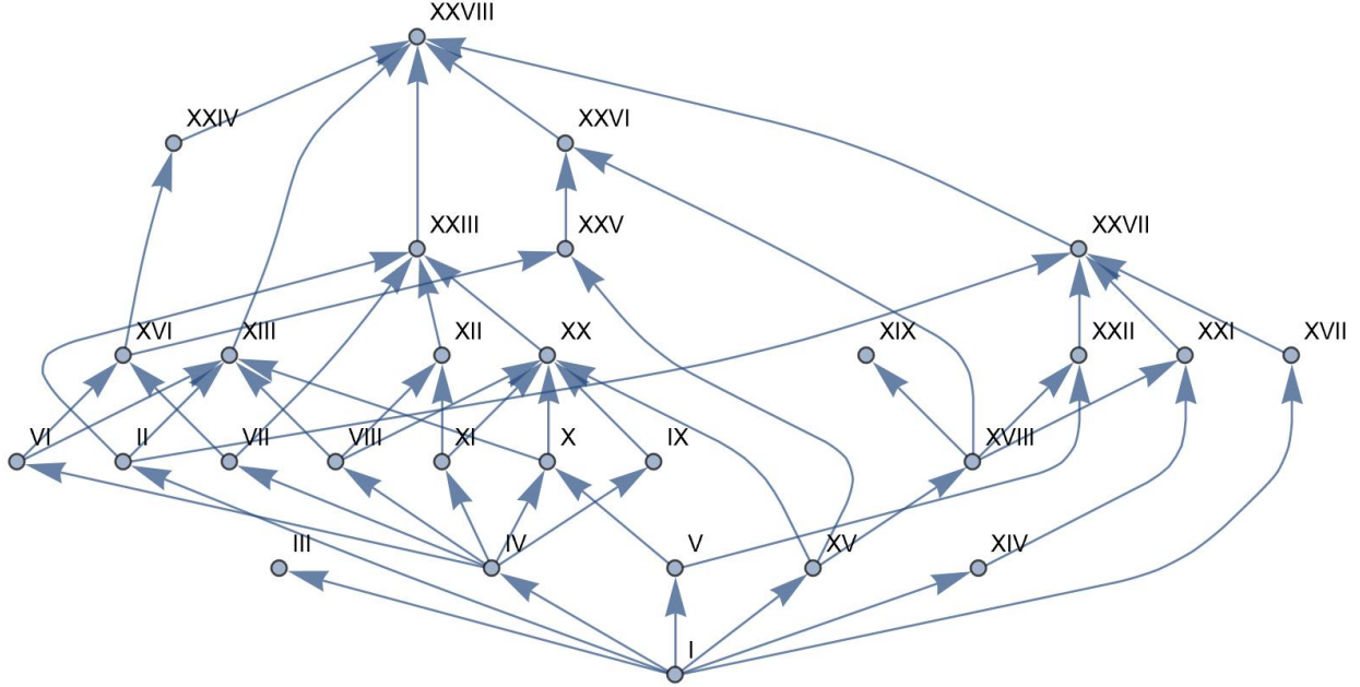
FIGURE 1. The grouping of eta quotients in Table 9, which have vanishing coefficient behaviour similar to f_1^6
