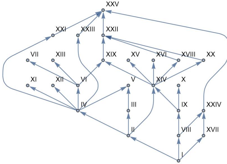
FIGURE 4. The grouping of eta quotients in Table 11, which have vanishing coefficient behaviour similar to f_1^8
