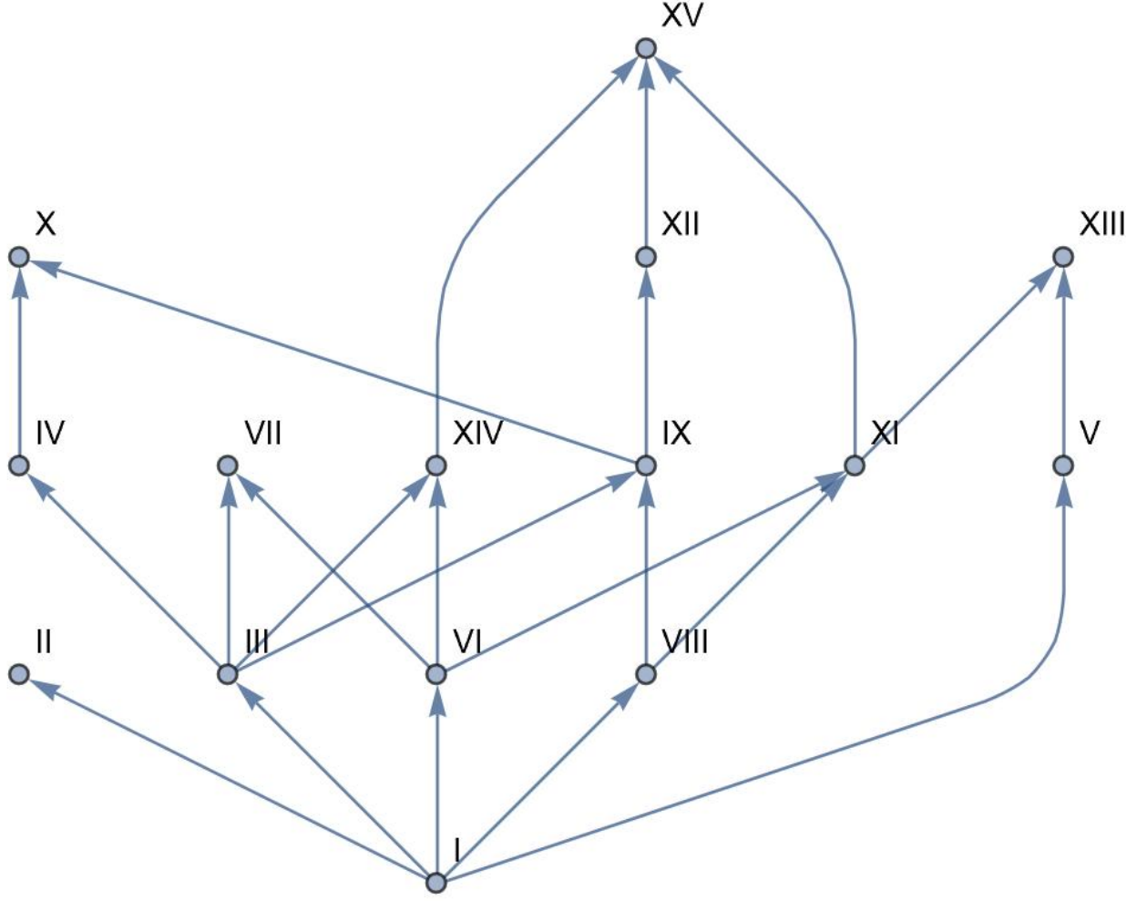
FIGURE 6. The grouping of eta quotients in Table 15, which have vanishing coefficient behaviour similar to f_1^{14}
