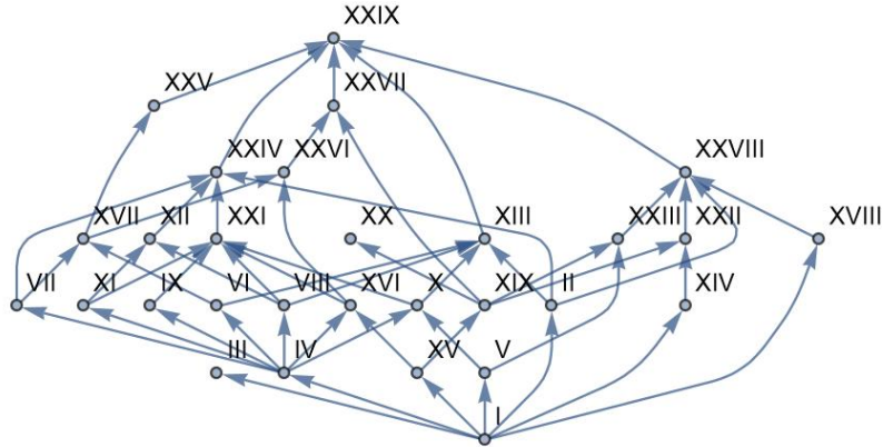
FIGURE 3. The grouping of eta quotients in Table 9, which have vanishing coefficient behaviour similar to f_1^6
