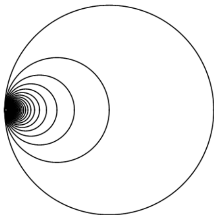
Infinite Earring Space
