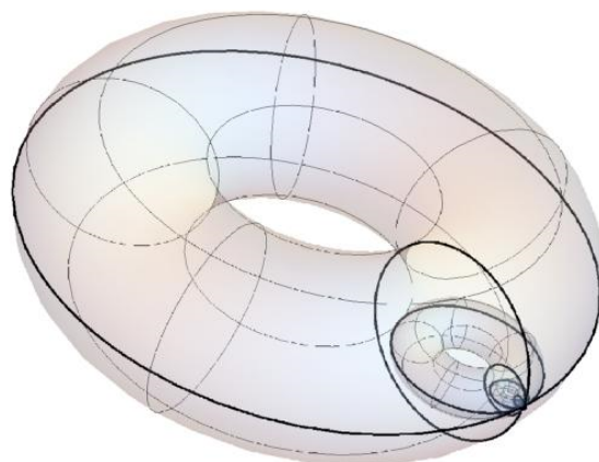
Shrinking Wedge of Tori
