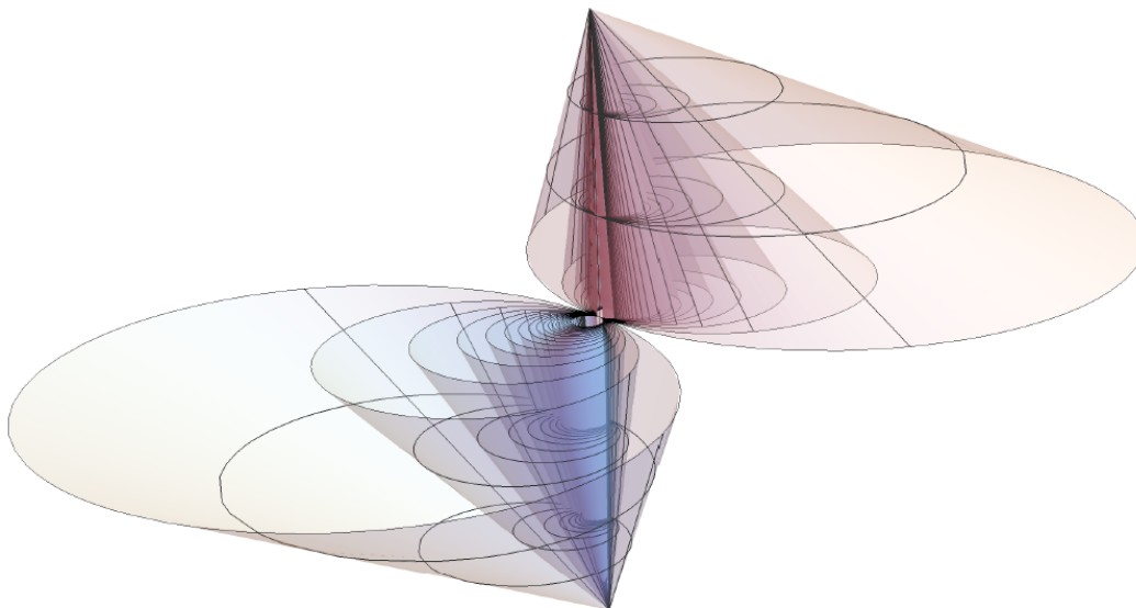
Griffiths Double Cone
